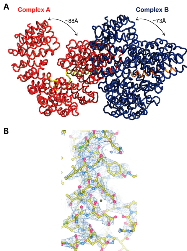
FIGURE 1: Conformational plasticity of importin \beta bound to the sIBB domain. (A) Asymmetric unit content with two importin \beta -sIBB domain complexes in different conformations shown as coils. Importin \beta is colored red and blue and the sIBB domain yellow and orange. (B) Representative 2F_o - F_c electron density computed at 3.15 Å resolution and contoured 1.5 \sigma above background. This figure was generated with Pymol (28).
