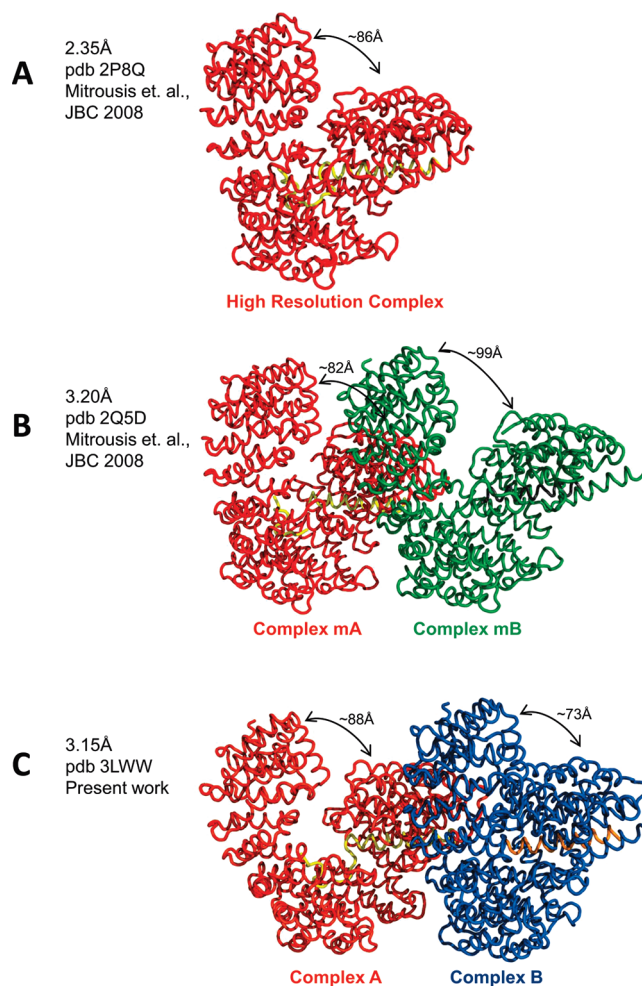
FIGURE 3: Comparison of the new crystal form with previously determined structures of the importin \beta -sIBB domain (residues 25–65) complex: (A) 2.35 Å structure (PDB entry 2P8Q) with one importin \beta -sIBB domain (residues 25–65) complex in the asymmetric unit, (B) 3.2 Å structure (PDB entry 2Q5D) with two importin \beta -sIBB domain (residues 25–65) complexes (indicated as mA-mB) in the same asymmetric unit, and (C) 3.15 Å structure presented in this paper (PDB entry 3LWW) with complexes A and B in the same asymmetric unit. All structures in panels A–C are aligned using importin \beta in complex A as a reference that is colored red.
